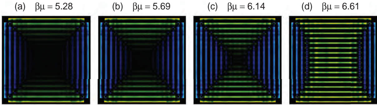
FIG. 8. (Color) Density false-color plots of confined structures in the case \kappa = 3 for fixed cavity size H = 7L . Cases for different chemical potential values (in the range \beta\mu = 5.28 – 6.61 ) are shown. Note that it is actually the product Q(\mathbf{r})\rho(\mathbf{r}) [see Eqs. (7) and (10)] that is plotted in the graphs, with the case \rho_y > \rho_x represented in blue (dark grey, vertical layers) and the case \rho_y < \rho_x represented in yellow (light grey, horizontal layers).
