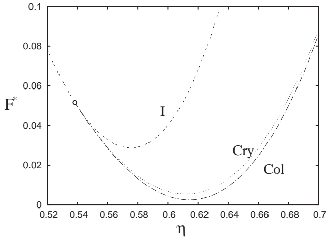
FIG. 3. Free-energy density branches in reduced units F^* = \beta \mathcal{F} L \sigma / A of the I , Col , and Cry phases with respect to packing fraction for the HR fluid with aspect ratio \kappa = 1 (hard squares). The straight line f = a\eta + b , with a = 6.20 and b = -3.22 , has been subtracted from the free energies in order to better visualize the curves. The transition point is located at \eta = 0.538 .
