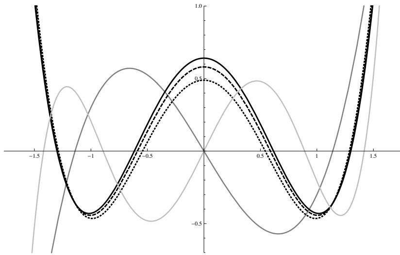
Figure 1: The graphs of Q_3^1(x) and Q_5^1(x) (gray) and Q_4^1(x) for some values of M (black lines).
