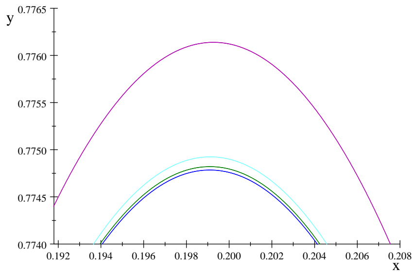
FIGURE 4. 16 - th partial sums, (Zoom), for \lambda = 0.1 (purple), 0.8 (cyan), 1.8 (green) and 10 (blue), when \eta = 1 , a = 1 , b = 3
