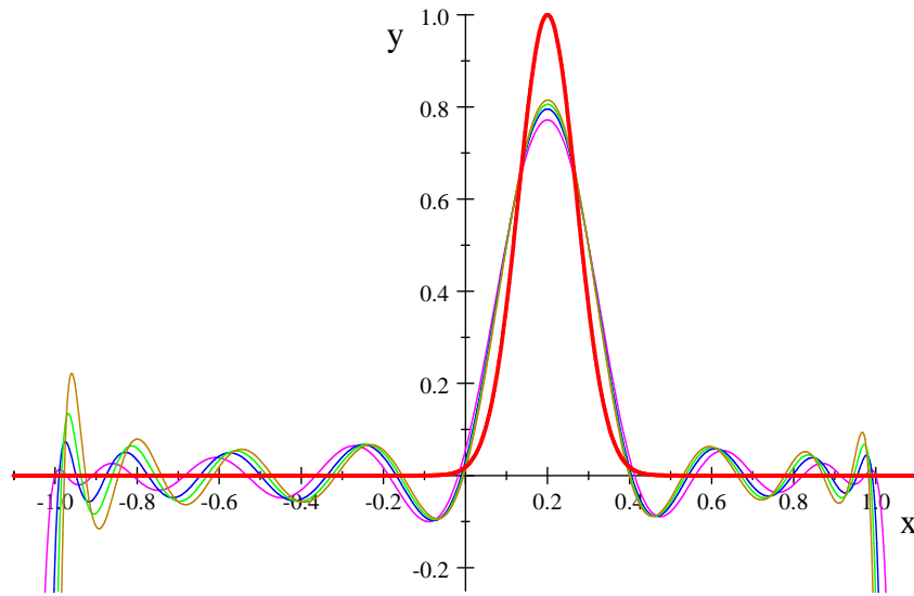
FIGURE 2. 16 - th partial sums for \eta = 0.5 (magenta), 1.5 (blue), 2 (green) and 2.5 (siena), when \lambda = 0.7 , a = 2 , b = 1 , f in red.
